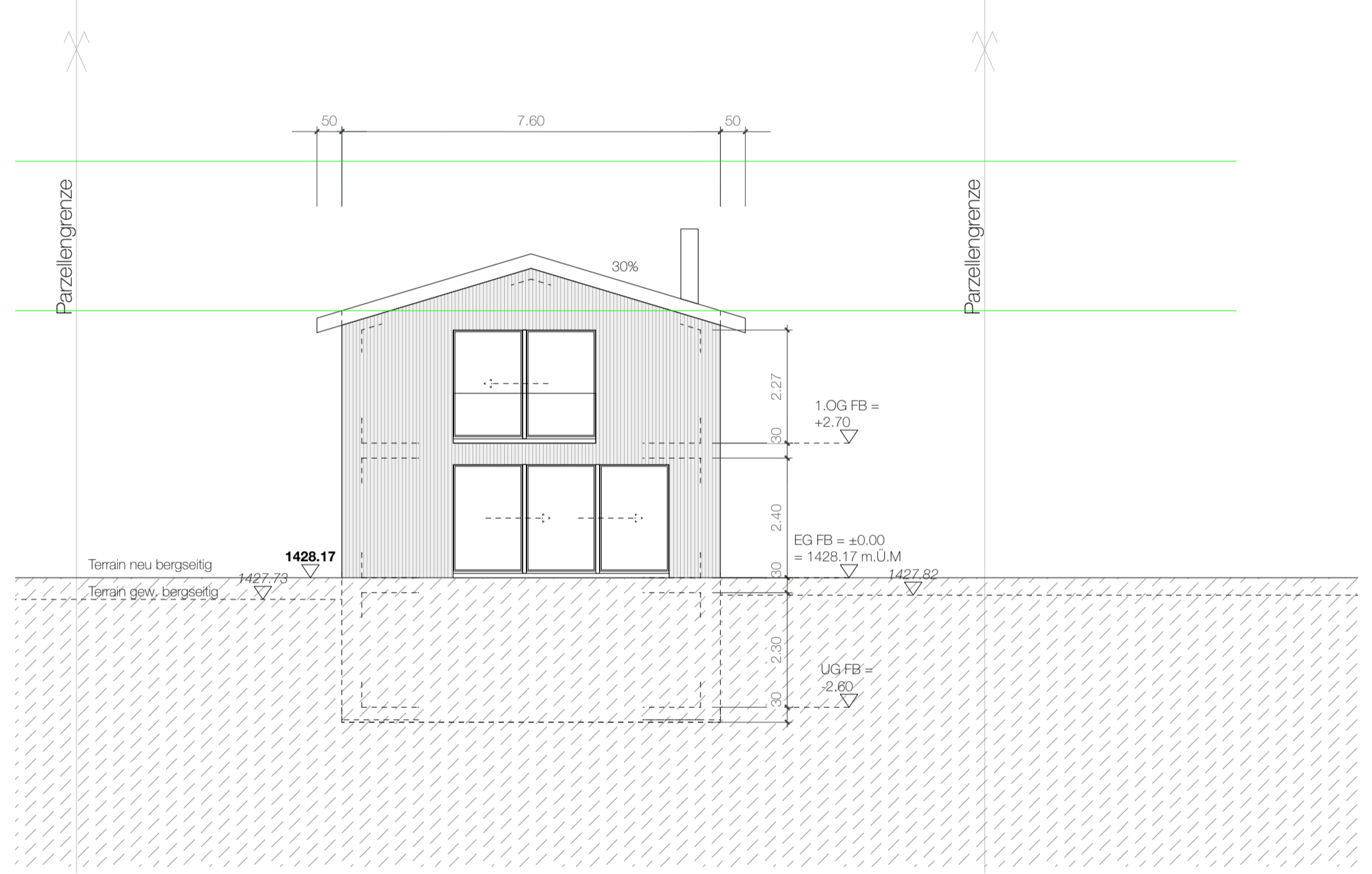
Fassade West I 1.100
